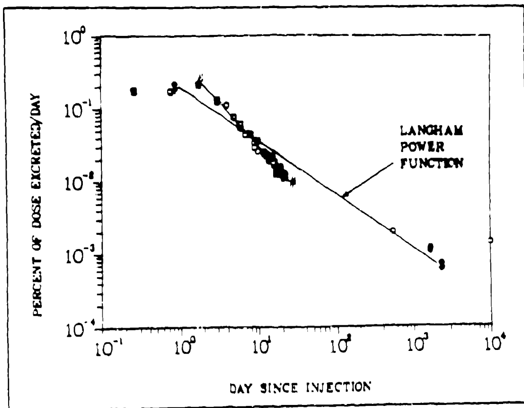
FIGURE 10. Excretion data for case HP-6. A power function curve for data collected on days 3-23 is shown by the solid line between the \bullet symbols. The power function for these data, days 2-23, where t = days of postexposure, is per cent excreted per day = 0.43t^{-1.24} , r = 0.99 . The Langham power function model through day 1750 is indicated by the solid line drawn between the \circ symbols.
